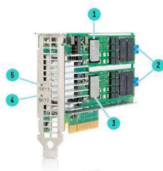
HPE NS204i-p Gen10+ Boot Device, half height
